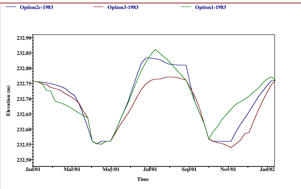
Chiblow Lake Water Levels For Options 1, 2c, and 3 Typical Wet Year 1983
