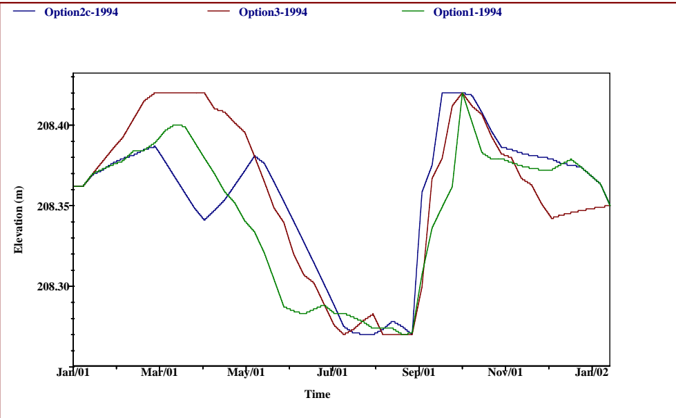
Scarfe (Canoe) Lake Water Levels For Options 1, 2c, and 3 Typical Average Year 1994
