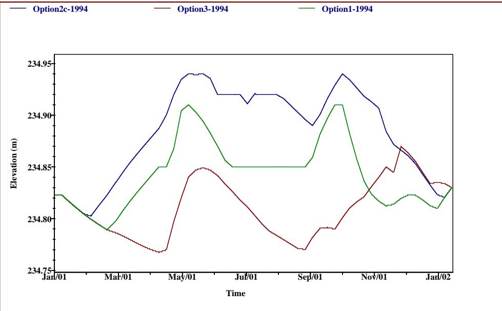
Matinenda Lake Water Levels For Options 1, 2c, and 3 Typical Average Year 1994
