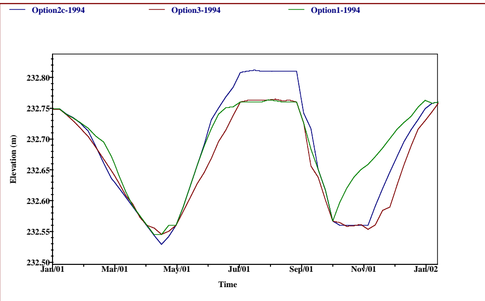
Chiblow Lake Water Levels For Options 1, 2c, and 3 Typical Average Year 1994
