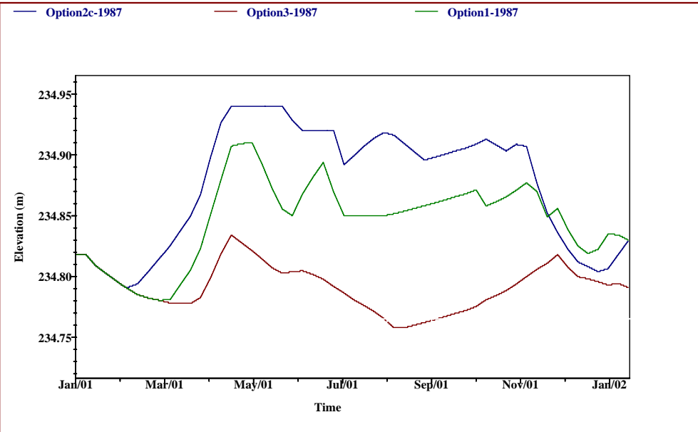
Matinenda Lake Water Levels For Options 1, 2c, and 3 Typical Dry Year 1987
