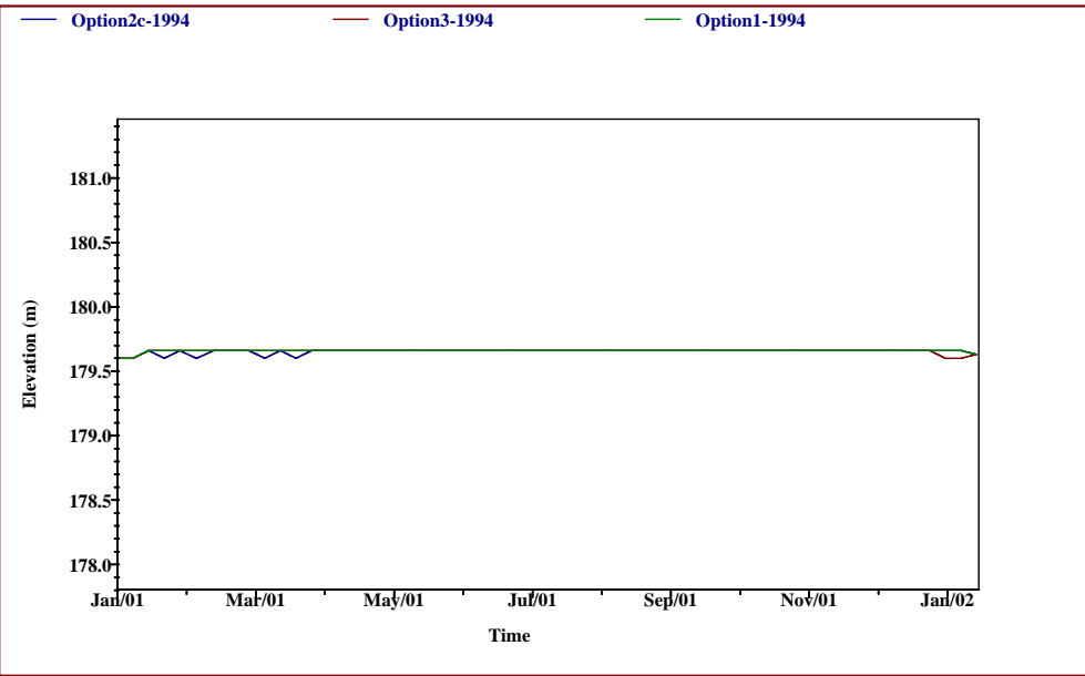
Lake Duborne Water Levels For Options 1, 2c, and 3 Typical Average Year 1994
