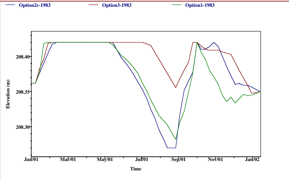
Scarfe (Canoe) Lake Water Levels For Options 1, 2c, and 3 Typical Wet Year 1983
