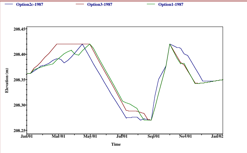
Scarfe (Canoe) Lake Water Levels For Options 1, 2c, and 3 Typical Dry Year 1987
