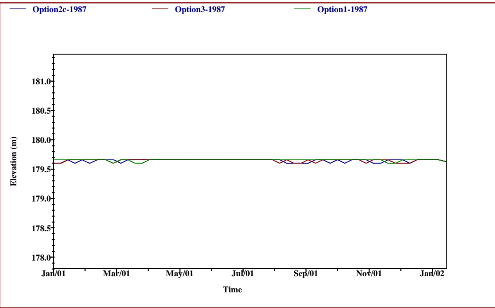
Lake Duborne Water Levels For Options 1, 2c, and 3 Typical Dry Year 1987
