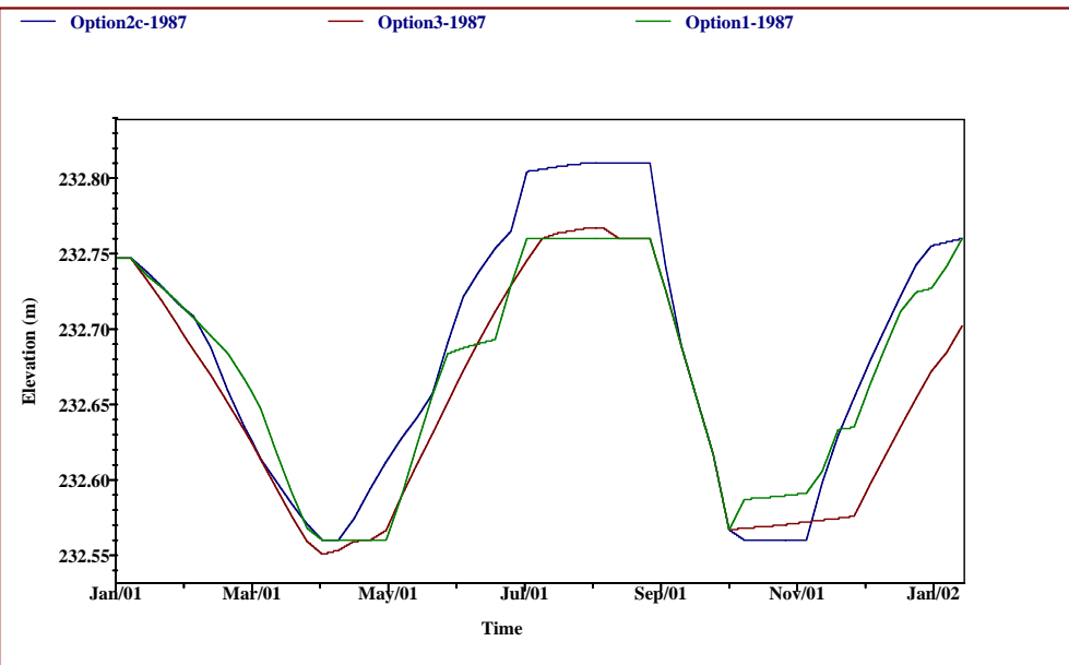
Chiblow Lake Water Levels For Options 1, 2c, and 3 Typical Dry Year 1987
